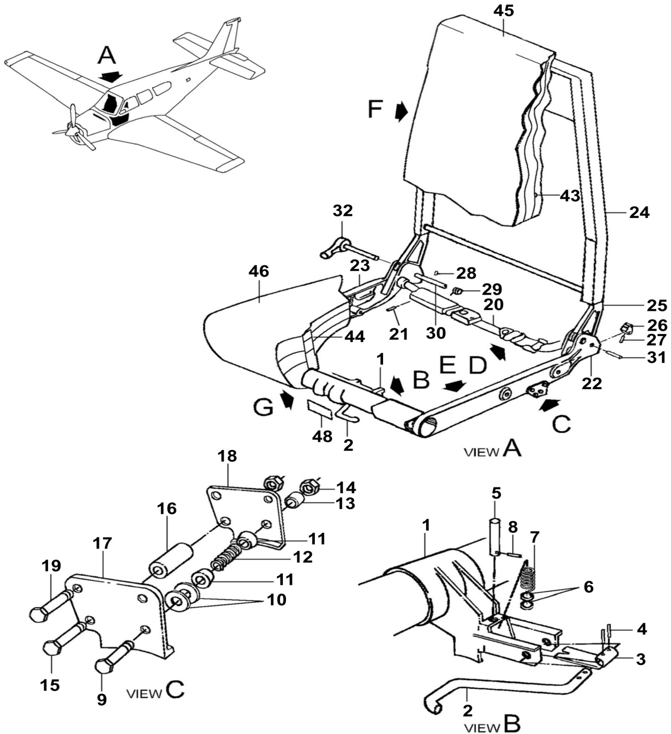
Figure 01 : Sheet 1 : PILOT AND COPILOT SEATS
