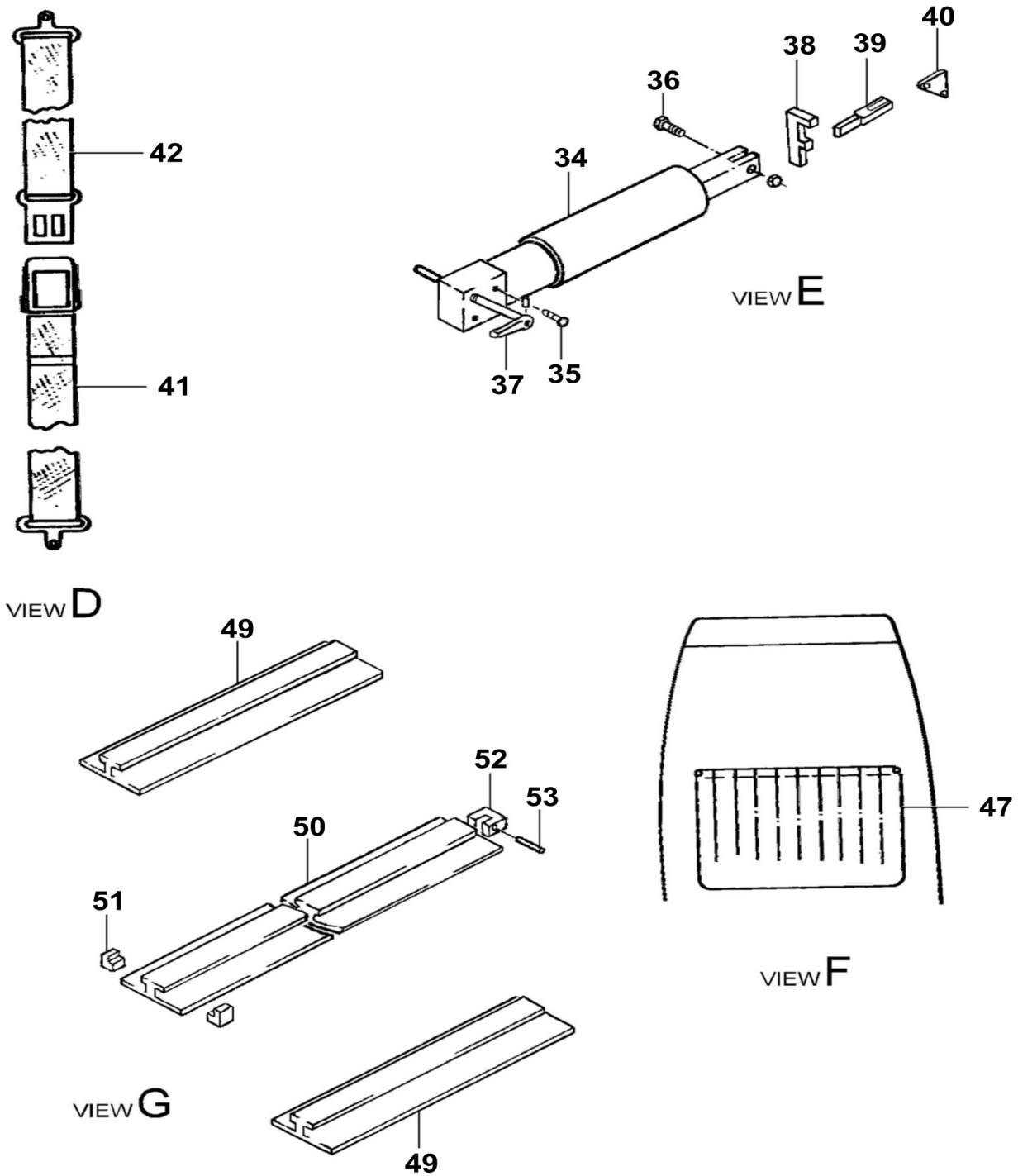
Figure 01 : Sheet 2 : PILOT AND COPILOT SEATS
